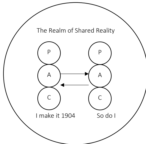
Figure 1 The Positivistic Universe
