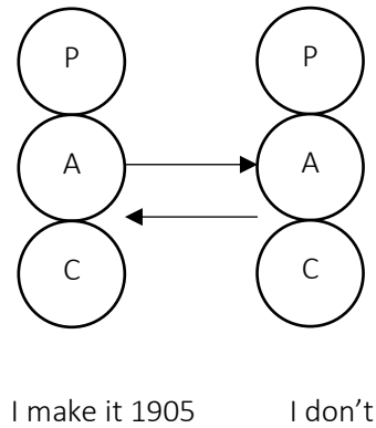
Figure 2 The Relativistic Universe
